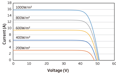
I-V CURVES OF PV MODULE (635W)
